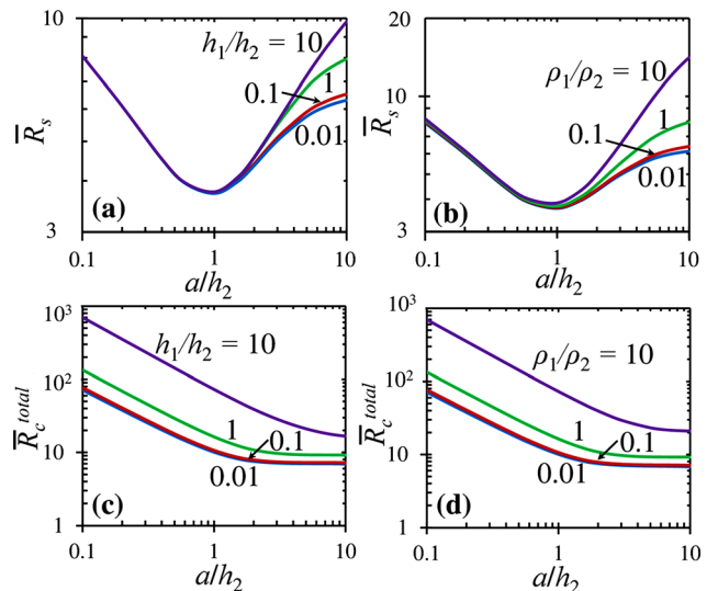
FIG. 4. (a) and (b) \bar{R}_s as a function of a/h_2 for various h_1/h_2 at \rho_1/\rho_2 = 1 , and for various \rho_1/\rho_2 at h_1/h_2 = 1 , respectively; (c) and (d) \bar{R}_c^{Total} as a function of a/h_2 for various h_1/h_2 at \rho_1/\rho_2 = 1 , and for various \rho_1/\rho_2 at h_1/h_2 = 1 , respectively.
