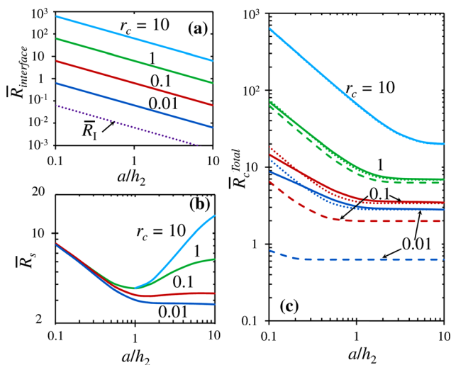
FIG. 2. (a) \bar{R}_{interface} , (b) \bar{R}_s , (c) \bar{R}_c^{Total} as function of a/h_2 , for various r_c = \rho_c / \rho_2 h_2 in Fig. 1(a). The TLM (dashed lines) and the ETLM (dotted lines) are shown in (c) for comparison.
