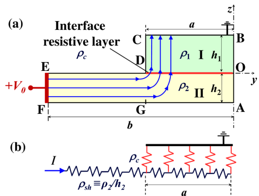
FIG. 1. (a) Electrical contact and (b) its TLM. In (a), an infinitesimally thin resistive interface layer is sandwiched between Regions I and II.
