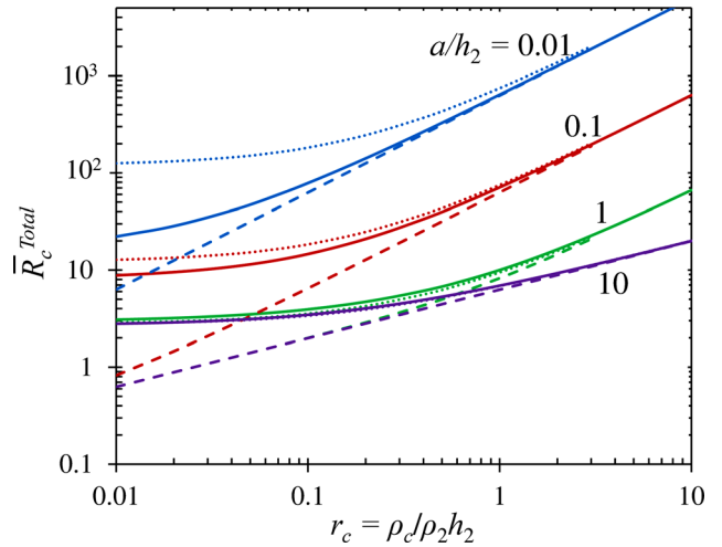
FIG. 3. \bar{R}_c^{Total} as a function of r_c = \rho_c / \rho_2 h_2 for various a/h_2 in Fig. 1(a), using the same set of parameters as Fig. 2. The dashed lines are for TLM, and the dotted lines are for ETLM.
