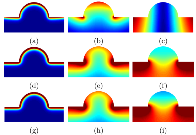
FIG. 9. Magnitude of the total electric field |\mathbf{E}| for the incident field \mathbf{H}_{02} in a region around the bump on the conducting plane of the same electric properties for \delta/a=0.1 (1st column), \delta/a=1 (2nd column), \delta/a=10 (3rd column), \lambda/a=10 (1st row), \lambda/a=100 (2nd row), and \lambda/a=1000 (3rd row).
