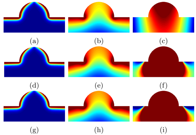
FIG. 7. Magnitude of the total electric field |\mathbf{E}| for the case \mathbf{E}_0 in a region around the bump on the conducting plane of the same electric properties for \delta/a=0.1 (1st column), \delta/a=1 (2nd column), \delta/a=10 (3rd column), \lambda/a=10 (1st row), \lambda/a=100 (2nd row), and \lambda/a=1000 (3rd row).
