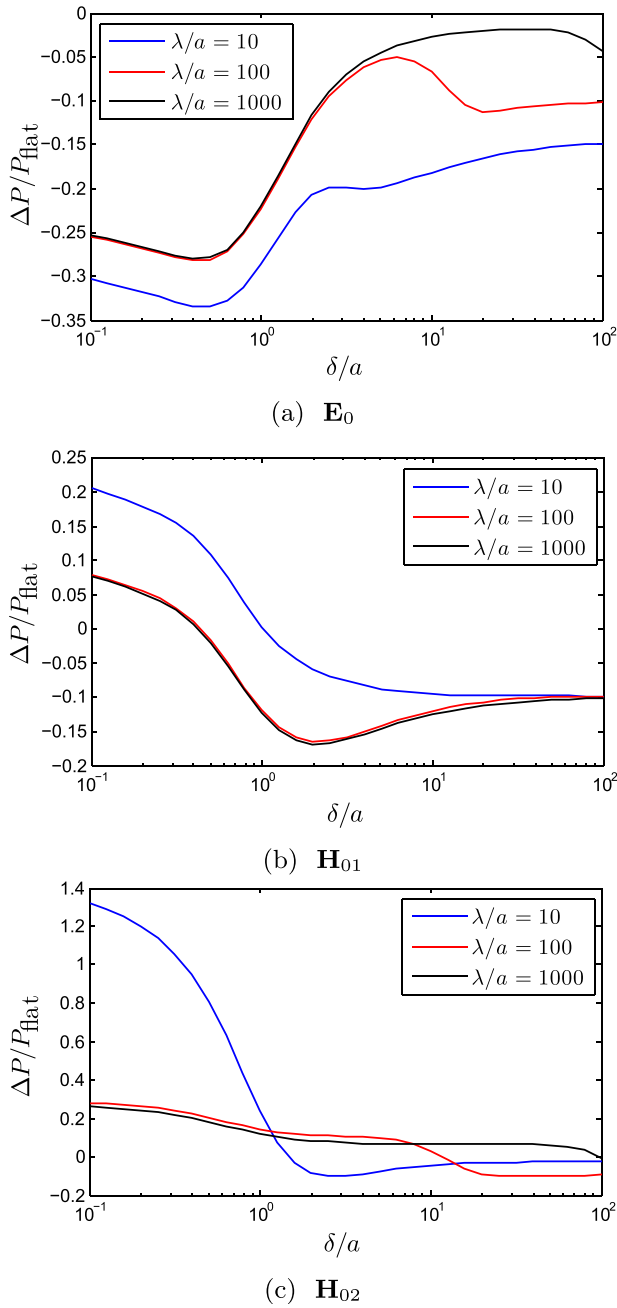
FIG. 6. \Delta P/P_{\text{flat}} for various values of the skin depth \delta/a computed using HIEM for the case of the trench on the plane of finite conductivity.
