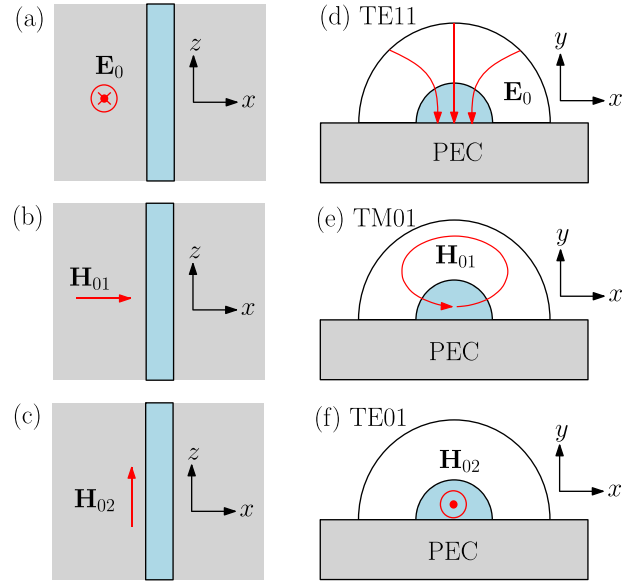
FIG. 2. Incident fields considered, following Ref. 5, for a bump on a PEC plane shown in Fig. 1. An incident electromagnetic field is either given by an electric field (a) \mathbf{E}_0 perpendicular to the PEC plane and associated magnetic field; by a magnetic field (b) \mathbf{H}_{01} parallel to the plane and perpendicular to the bump axis and associated electric field; or by a magnetic field (c) \mathbf{H}_{02} parallel to the bump axis and associated electric field. According to Ref. 5, these incident fields are approximated by (semi-)cylindrical eigenmodes, namely the (d) TE 11 mode, (e) TM 01 mode, and (f) TE 01 mode, respectively, which can themselves be expressed in closed-form in terms of products of Bessel functions and complex exponentials.
