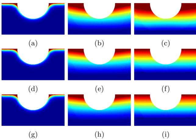
FIG. 11. Magnitude of the total electric field |E| for the incident field H_{01} in a region around the trench on the conducting plane of the same electric properties for \delta/a=0.1 (1st column), \delta/a=1 (2nd column), \delta/a=10 (3rd column), \lambda/a=10 (1st row), \lambda/a=100 (2nd row), and \lambda/a=1000 (3rd row).
