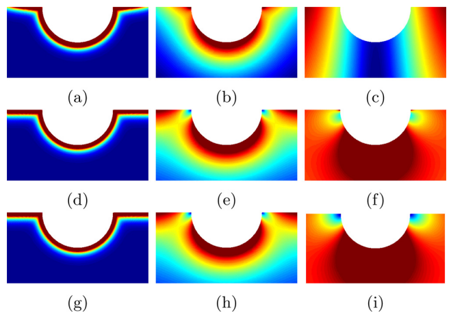
FIG. 12. Magnitude of the total electric field |E| for the incident field H_{02} in a region around the trench on the conducting plane of the same electric properties for \delta/a=0.1 (1st column), \delta/a=1 (2nd column), \delta/a=10 (3rd column), \lambda/a=10 (1st row), \lambda/a=100 (2nd row), and \lambda/a=1000 (3rd row).
