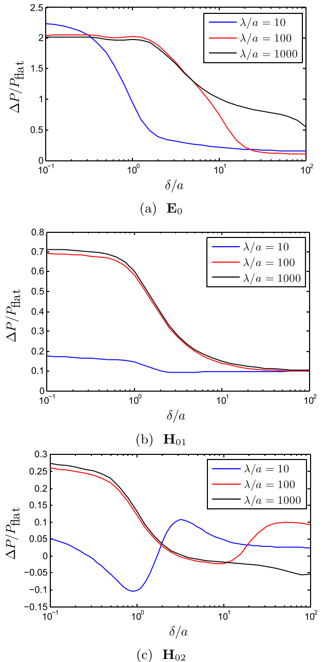
FIG. 5. \Delta P/P_{\text{flat}} for various values of \delta/a computed using HIEM for the case of the bump on the plane of finite conductivity.
