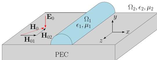
FIG. 1. A small semi-cylindrical bump on a perfectly conducting surface whose local wave electric field is \mathbf{E}_0 and local wave magnetic field \mathbf{H}_0 in the absence of the bump.
