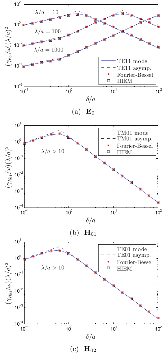
FIG. 4. (a) \gamma_{E_0} (Eq. (A2)) and its asymptotes (Eq. (A3)), (b) \gamma_{H_{01}} (Eq. (A5)) and its asymptotes (Eq. (A6)), and (c) \gamma_{H_{02}} (Eq. (A8)) and its asymptotes (Eq. (A9)), in terms of (\lambda/a)^2 , as a function of \delta/a for a number of values of \lambda/a , for the special case \mu_1 = \mu_2 = \mu_0 and \epsilon_{1r} = \epsilon_2 = \epsilon_0 . Red dots represent the exact value computed using the Fourier-Bessel expansion 32 of the exact solution of the problem of scattering, and the black squares represent the values obtained using HIEM.
