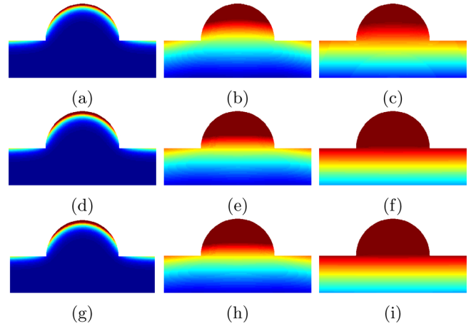
FIG. 8. Magnitude of the total electric field |\mathbf{E}| for the incident field \mathbf{H}_{01} in a region around the bump on the conducting plane of the same electric properties for \delta/a=0.1 (1st column), \delta/a=1 (2nd column), \delta/a=10 (3rd column), \lambda/a=10 (1st row), \lambda/a=100 (2nd row), and \lambda/a=1000 (3rd row).
