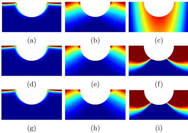
FIG. 10. Magnitude of the total electric field |E| for the incident field E_0 in a region around the trench on the conducting plane of the same electric properties for \delta/a=0.1 (1st column), \delta/a=1 (2nd column), \delta/a=10 (3rd column), \lambda/a=10 (1st row), \lambda/a=100 (2nd row), and \lambda/a=1000 (3rd row).
